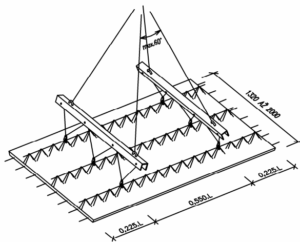
UCHYTENIE VAHADLAMI
