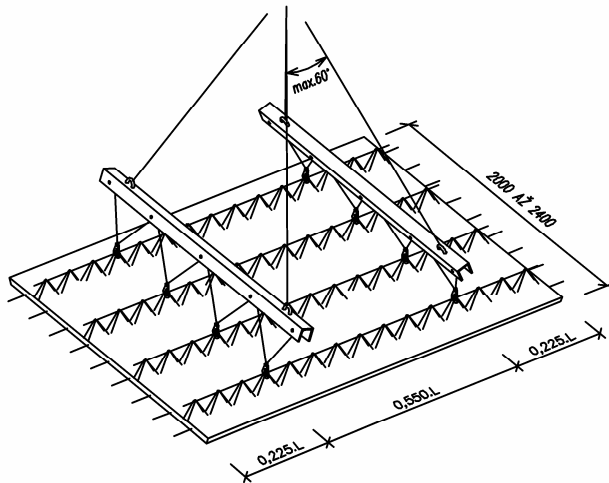
UCHYTENIE VAHADLAMI
