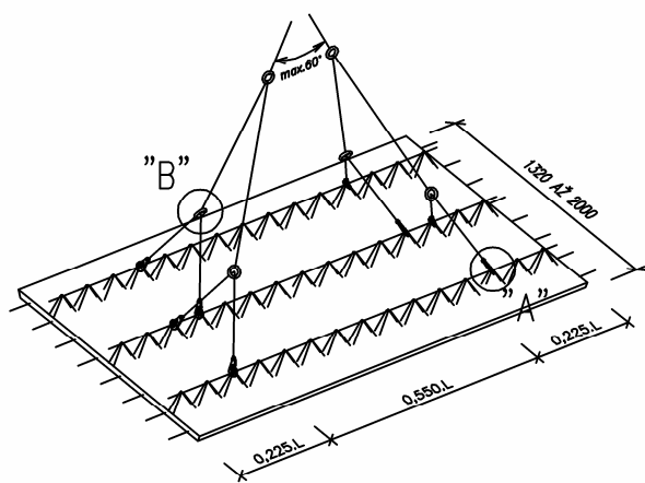
UCHYTENIE LANAMI
